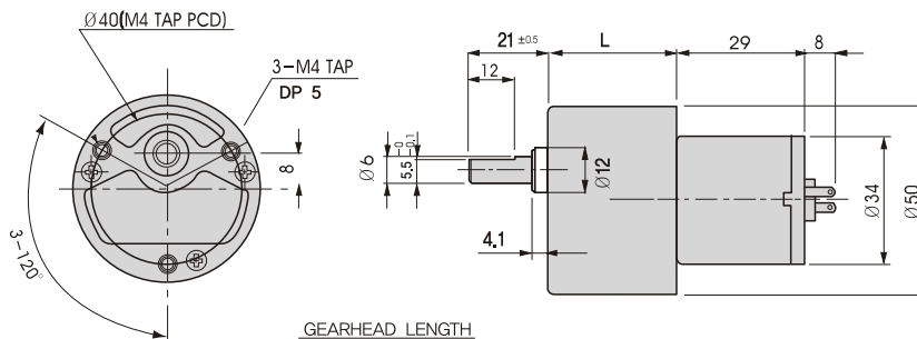
GEARHEAD LENGTH
