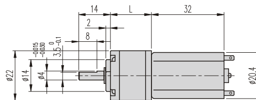
GEARHEAD LENGTH
