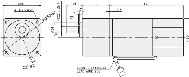
K9IP90F□-SU + K9P□B
