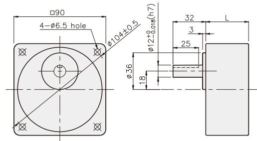
GEARHEAD K9G□B(C)
