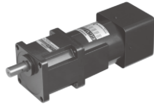
K9IP120F□-SU + K9P□BU
