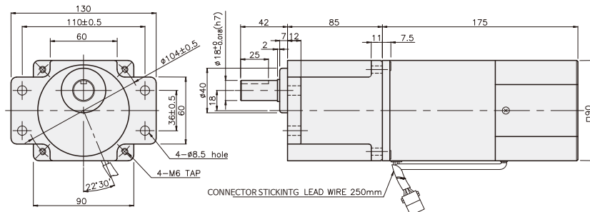
K9RP90F□-SU + K9P□BUF
