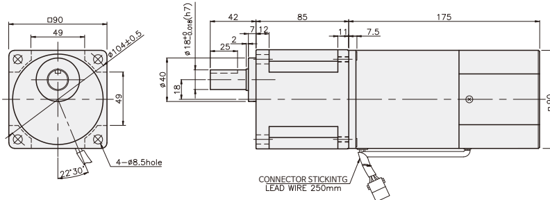
K9RP90F□-SU + K9P□BU
